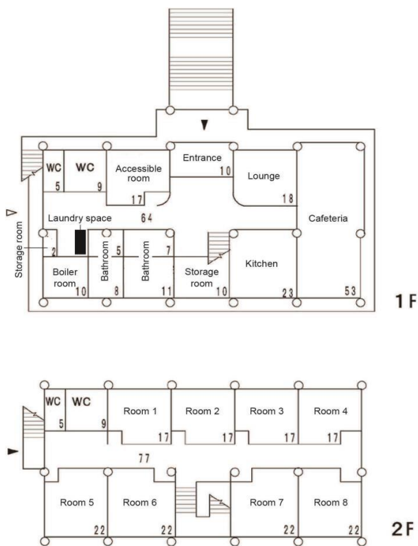
Fig 2. Floor plan.
